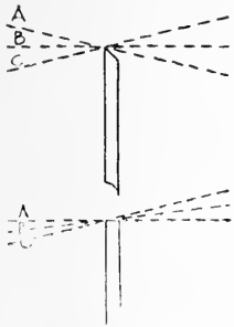
FIG. 120. ANGLE OF BURNISHER IN TURNING A BURR.
